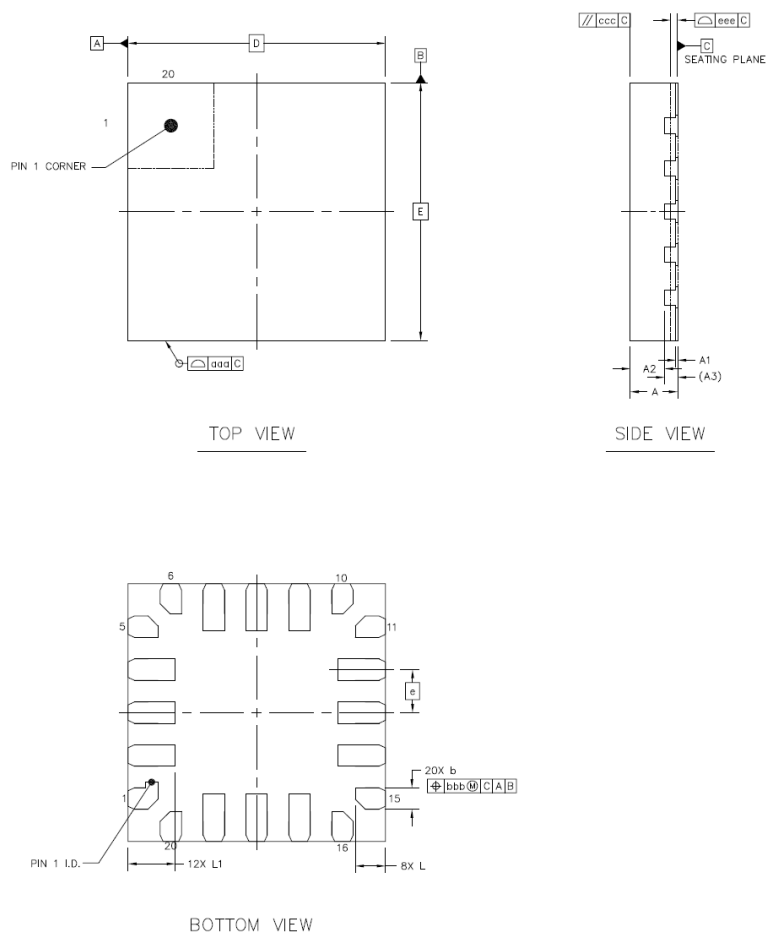
Figure 18 Package diagram of QFN20
