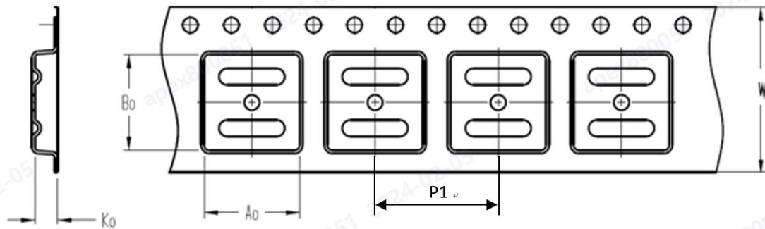
Figure 19 Tape Dimensions
